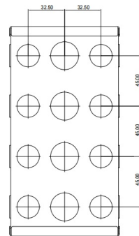
4 BACK VIEW
