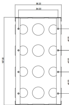
1 FRONT VIEW
