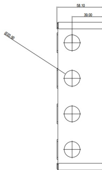
2 RIGHT VIEW
