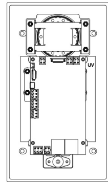
4 BACK VIEW
