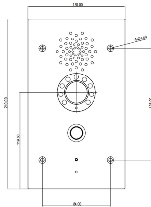
1 FRONT VIEW
