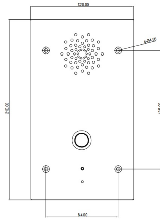
1 FRONT VIEW
