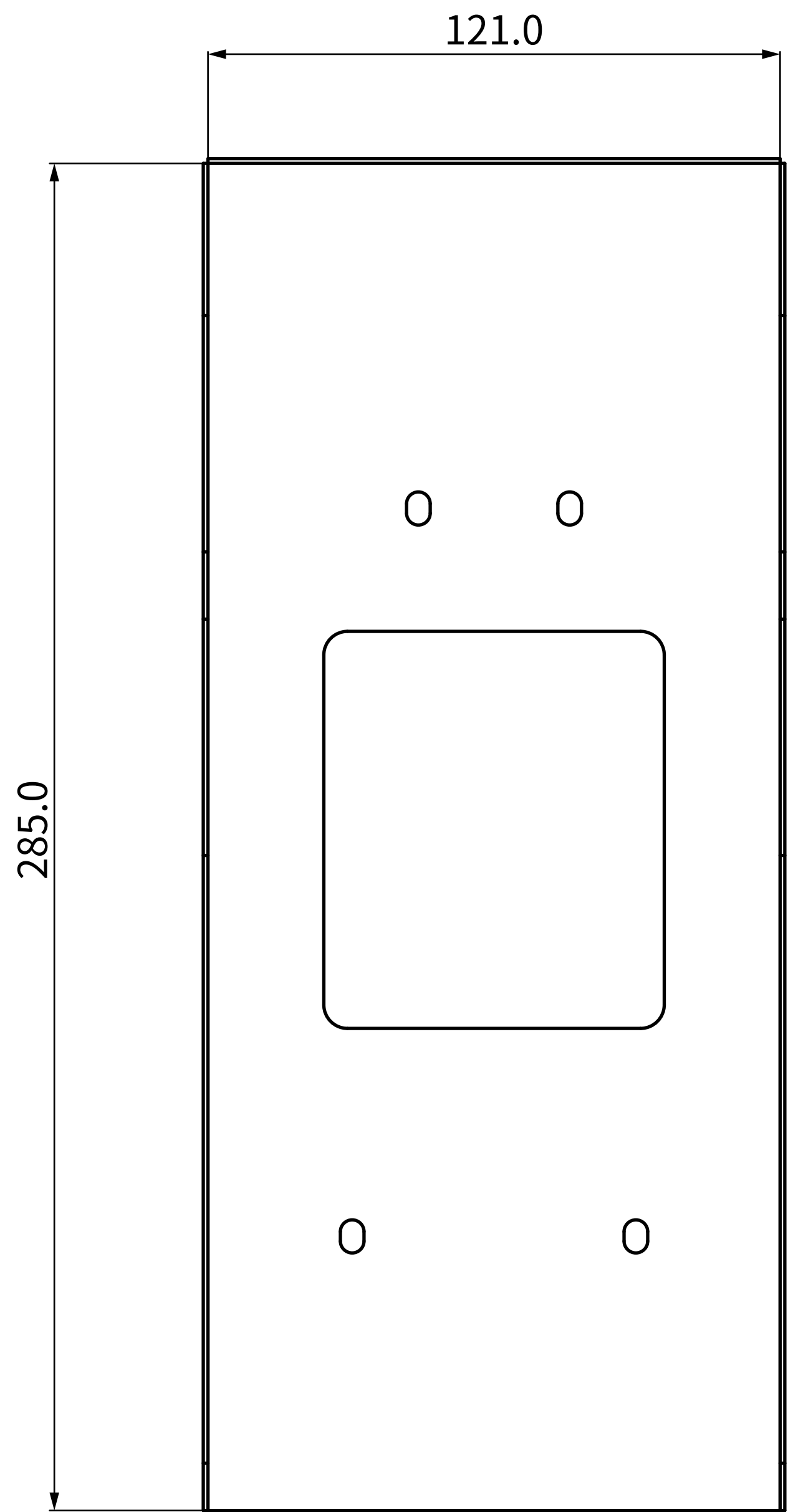
1 FRONT VIEW
