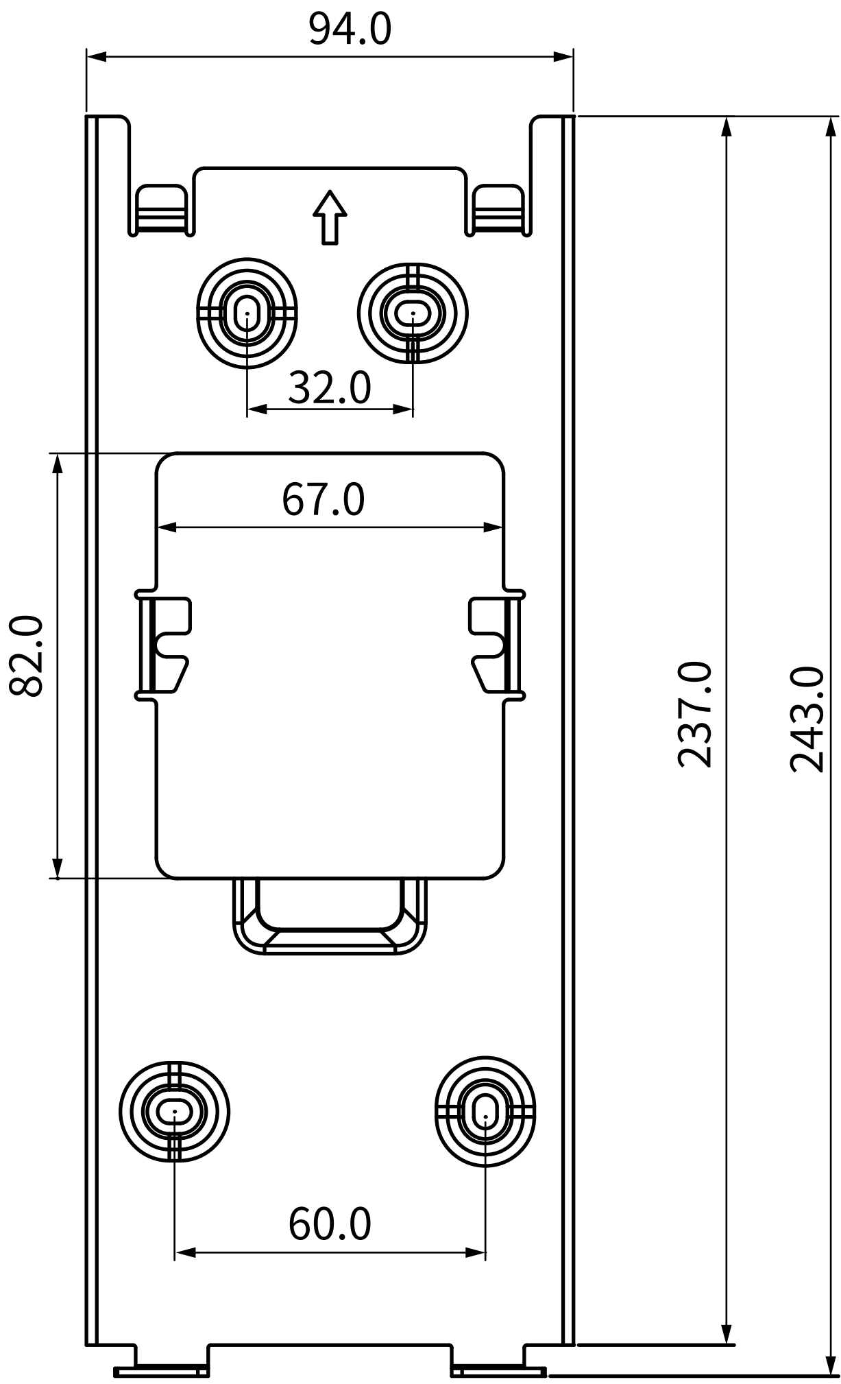
1 FRONT VIEW
