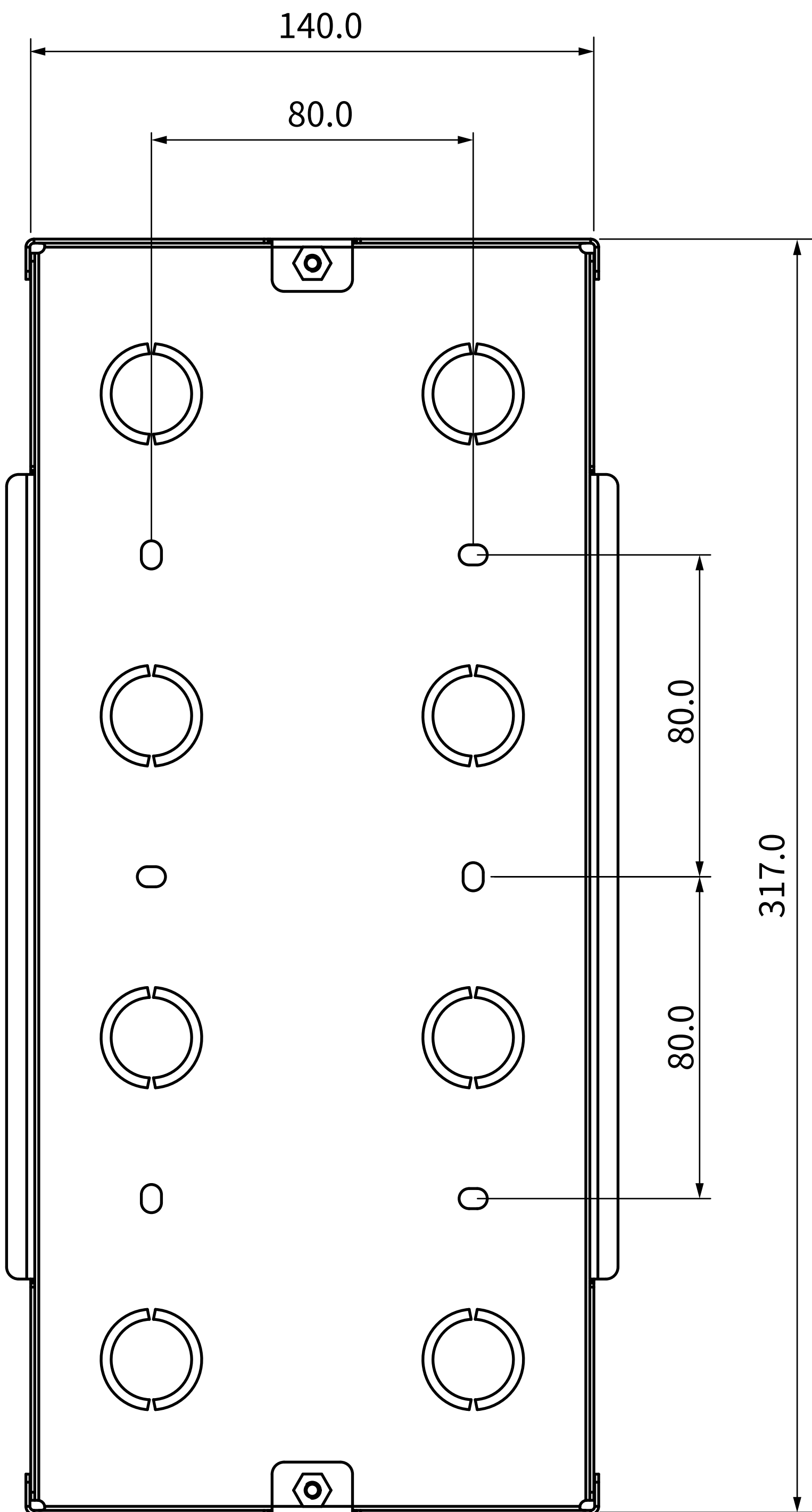
1 FRONT VIEW
