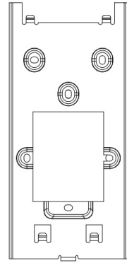
4 BACK VIEW
