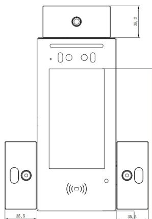
1 INTERCOM PANEL FRONT VIEW
