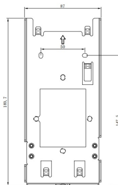
2 FRONT VIEW: WALL MOUNTING BRACKET PLACEMENT
