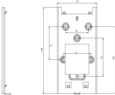
1 FRONT VIEW
