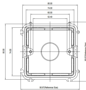
1 FRONT VIEW
