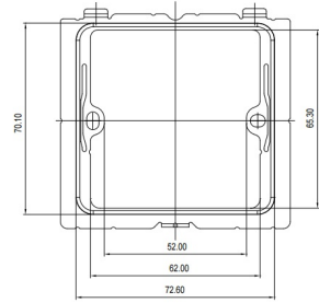
4 BACK VIEW
