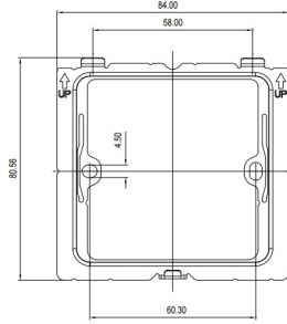
1 FRONT VIEW
