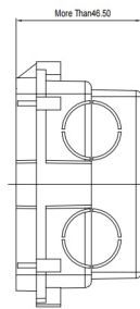
3 LEFT VIEW
